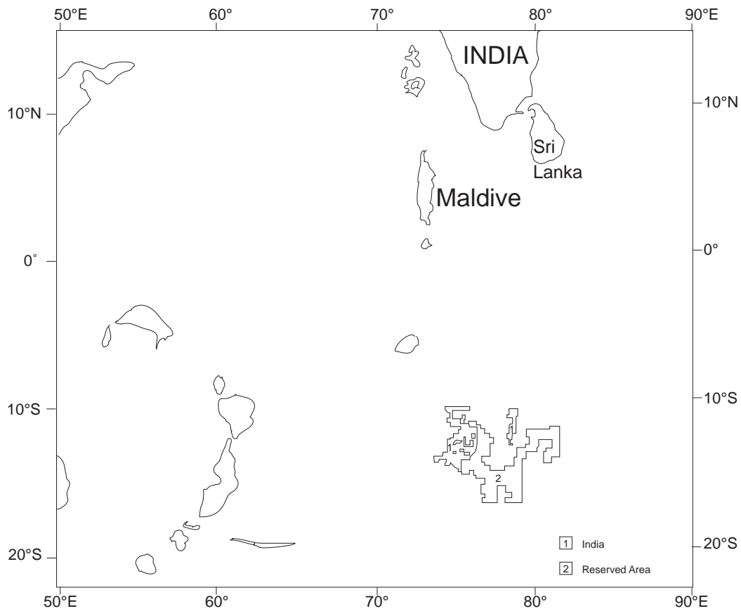
Fig. 2: Areas allotted to Pioneer Investors in the Pacific Ocean (above) and Indian Ocean (below) (modified from: www.isa.org.jm )
